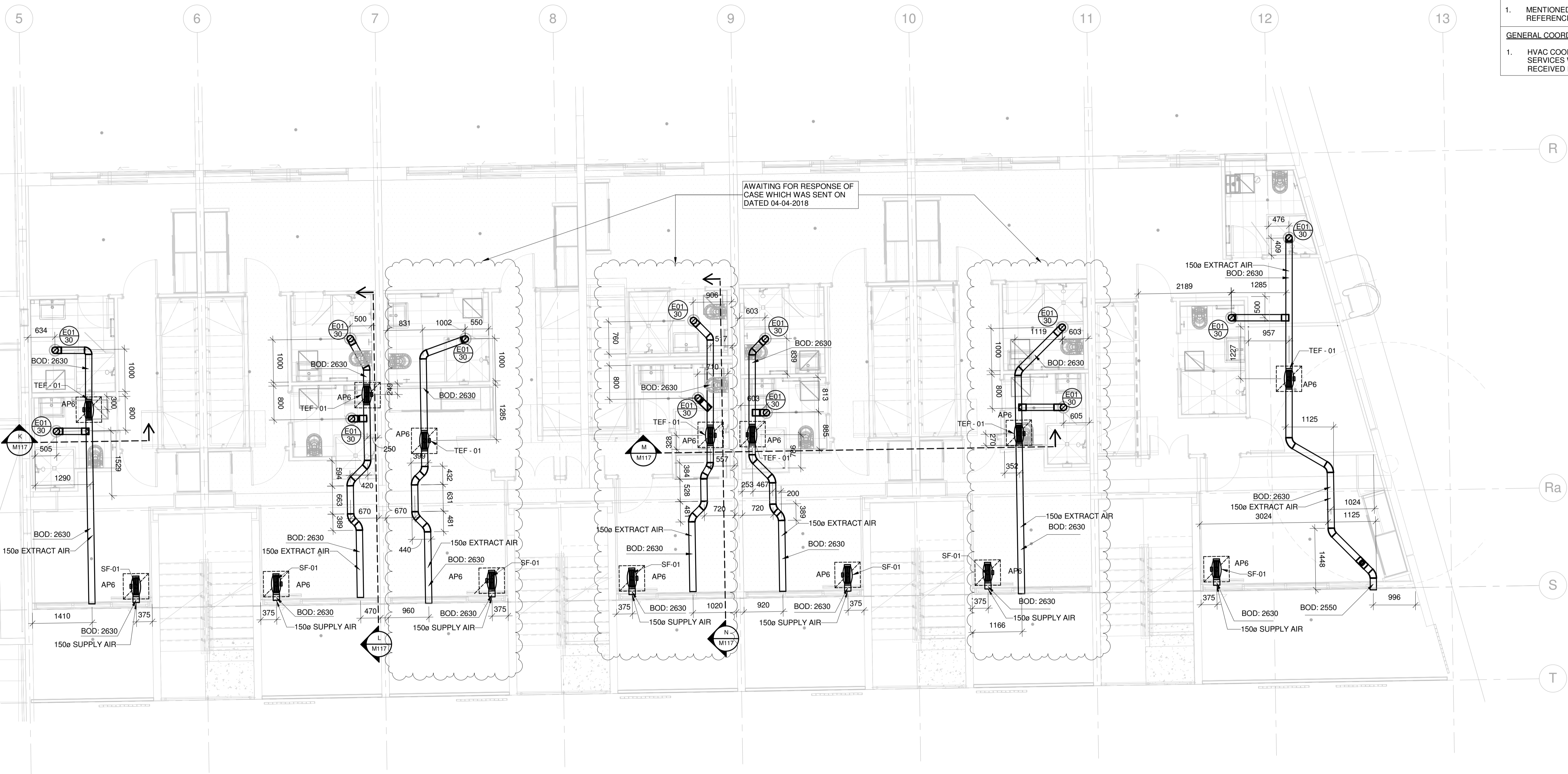
8 GROUND FLOOR BLOCK B HVAC LAYOUT M116 SCALE : 1 : 50
