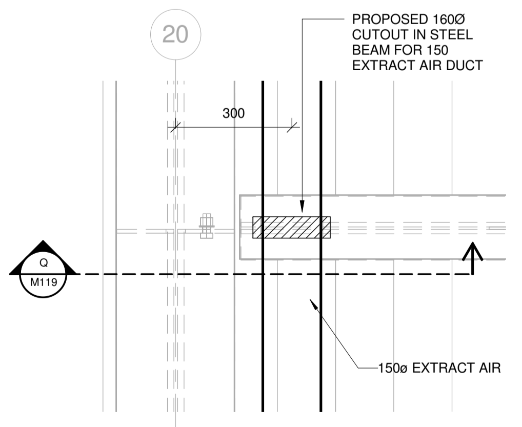
11 PROPOSED CUTOUT ENLARGE VIEW M119 SCALE : 1 : 10
