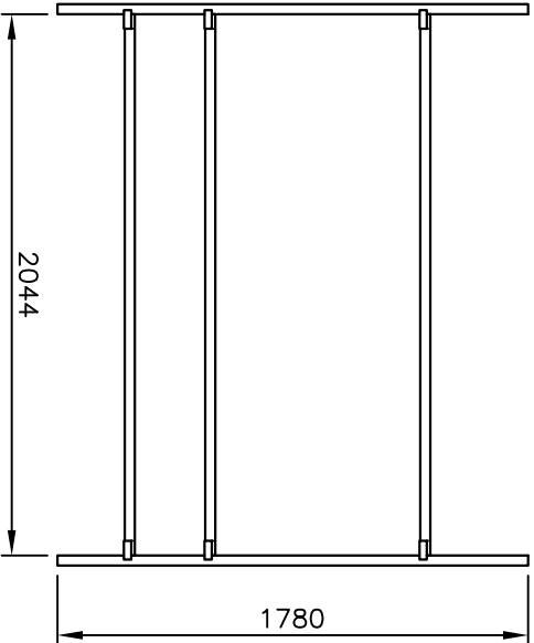
Front view of set up Lofted Bed with support rails.
