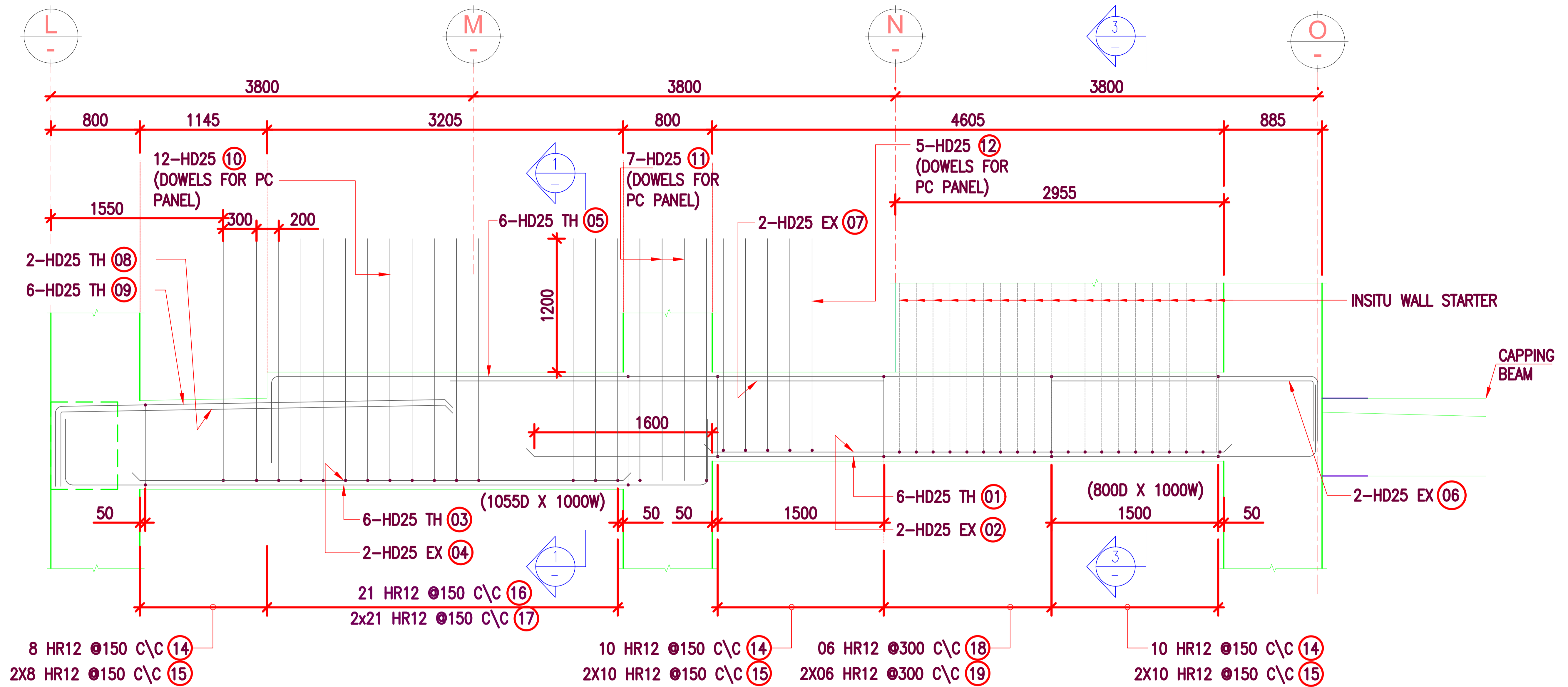
Beam Elevation Grid Line 27 (Ground Floor) (SCALE-1:20)
