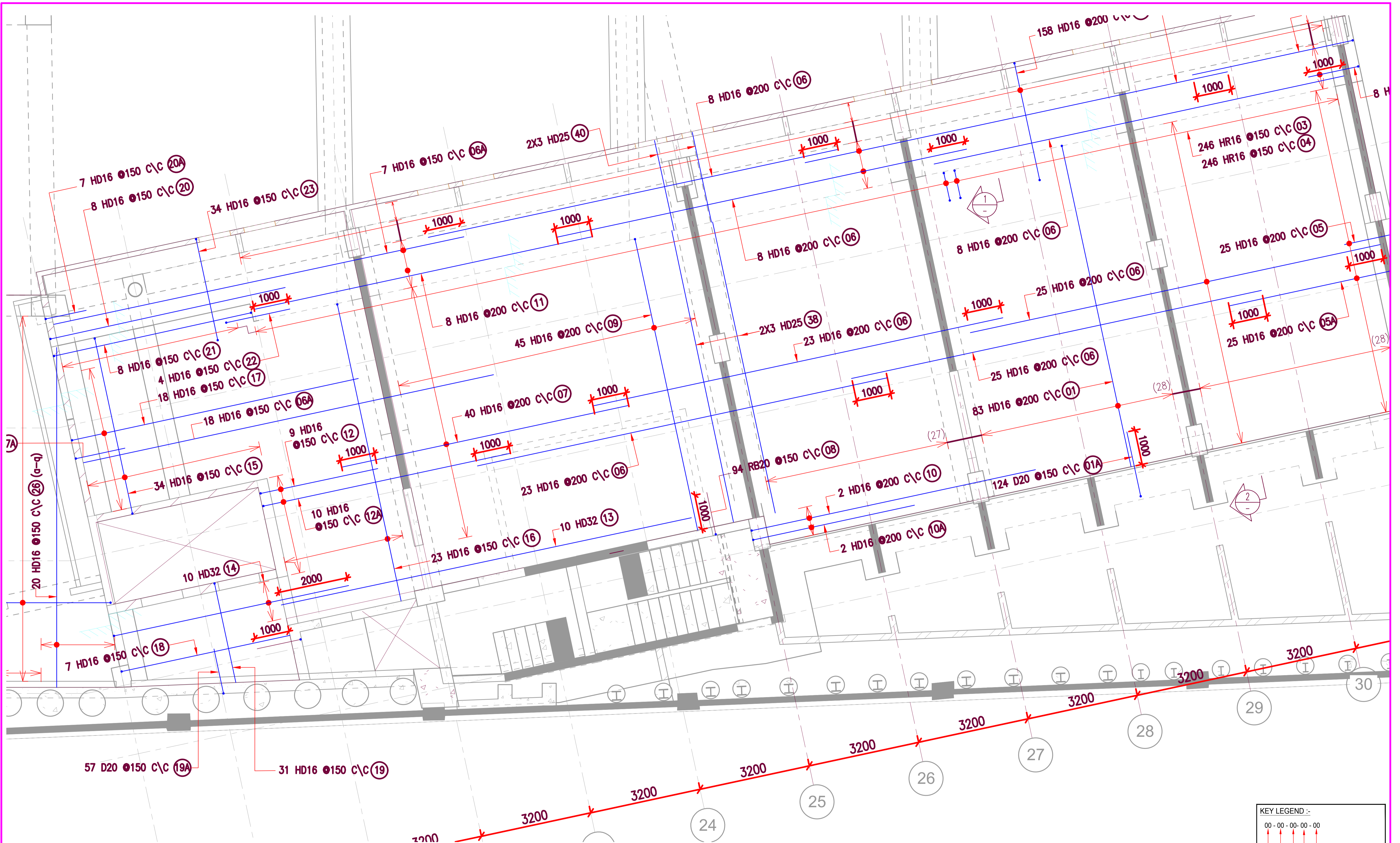
GROUND FLOOR SLAB LAYOUT (SCALE-1:100)
