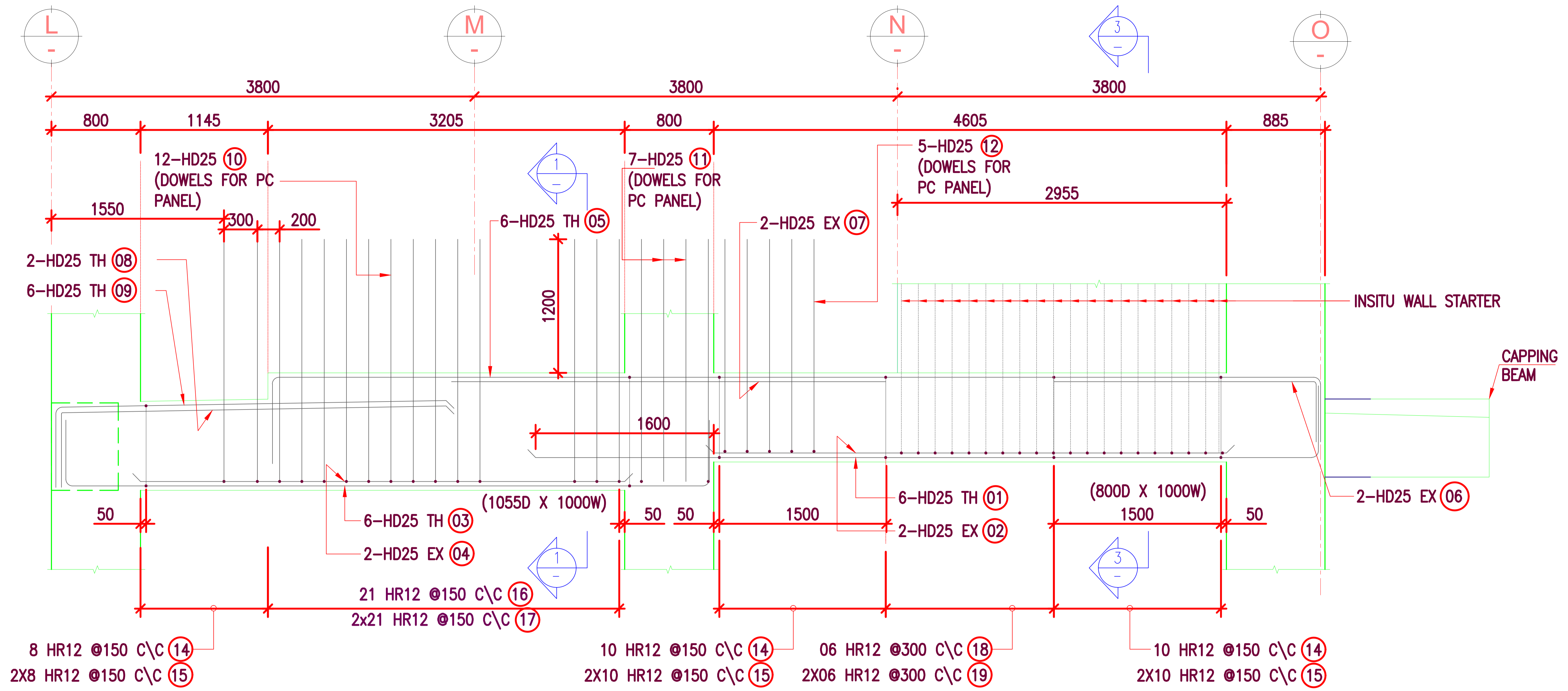
Beam Elevation Grid Line 27 (Ground Floor) (SCALE-1:50)
